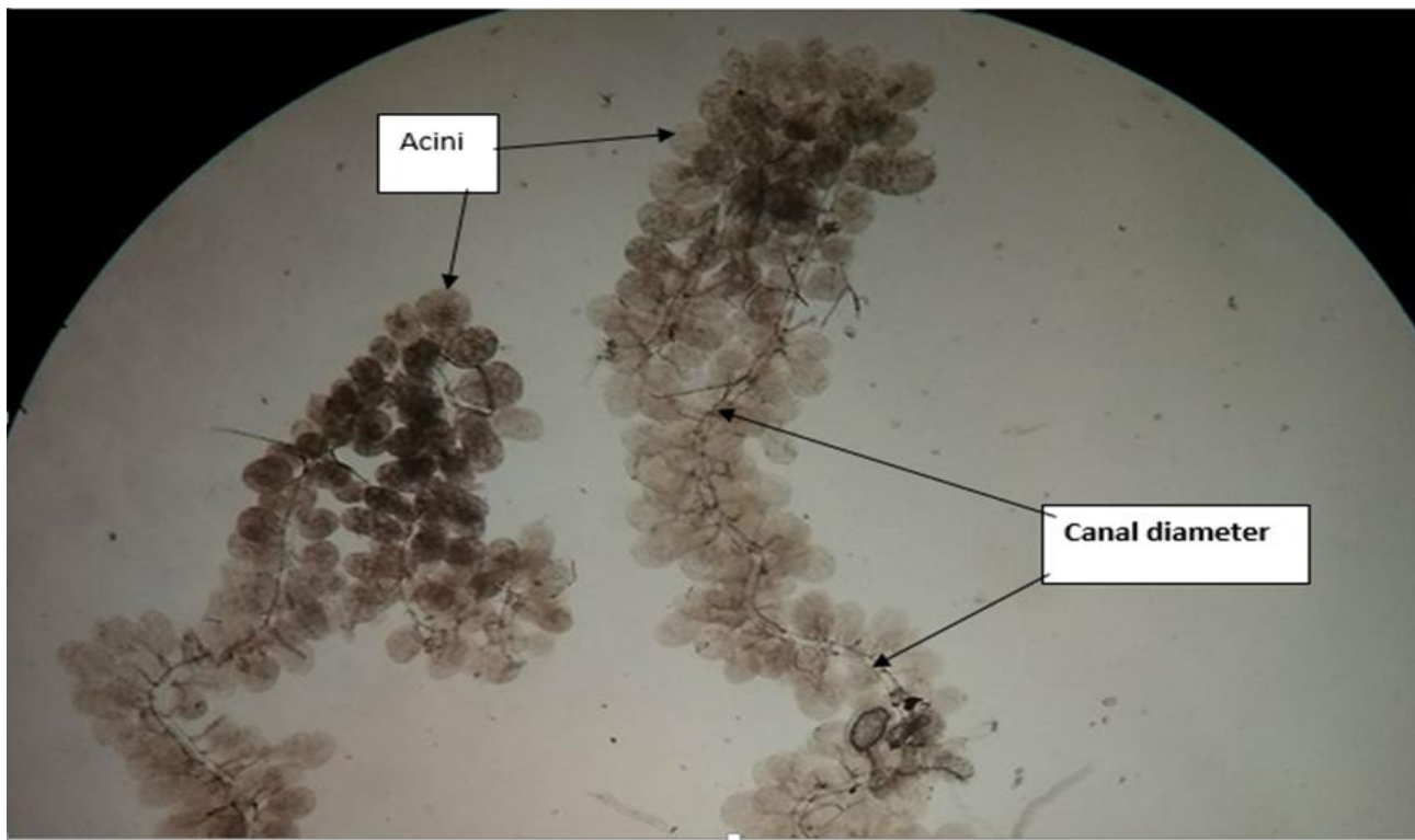
Fig.2 Hypopharyngeal gland of Honey bee worker (18 days old) reared on magnetized water. The number of acini and diameter of hypopharyngeal canals appear significantly higher than the control (Control in Fig.1)
